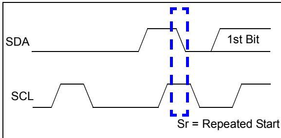
FIGURE B-5: Repeat Start Condition Waveform.
