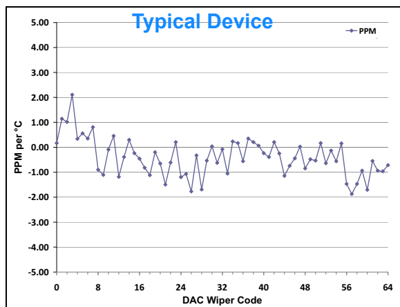
FIGURE 2-57: V_{OUT} Tempco vs. Code ( ((V_{OUT(+125C)} - V_{OUT(-40C)}) / V_{OUT(+25C, \text{Code}=FS)}) / 165) * 1,000,000 ), V_{DD} = 5.5\text{V} , V_{REF} = 1.65\text{V} .
