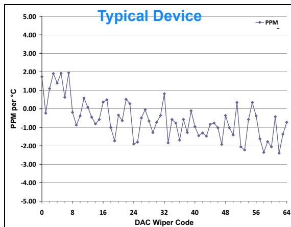
FIGURE 2-58: V_{OUT} Tempco vs. Code ( ((V_{OUT(+125C)} - V_{OUT(-40C)}) / V_{OUT(+25C, \text{Code}=FS)}) / 165) * 1,000,000 ), V_{DD} = 5.5\text{V} , V_{REF} = 1.0\text{V} .
