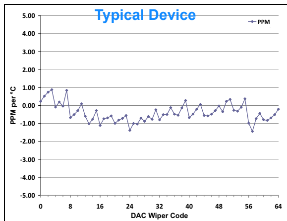
FIGURE 2-56: V_{OUT} Tempco vs. Code ( ((V_{OUT(+125C)} - V_{OUT(-40C)}) / V_{OUT(+25C, \text{Code}=FS)}) / 165) * 1,000,000 ), V_{DD} = 5.5\text{V} , V_{REF} = 5.5\text{V} .
