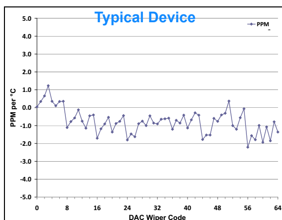
FIGURE 2-59: V_{OUT} Tempco vs. Code ( ((V_{OUT(+125C)} - V_{OUT(-40C)}) / V_{OUT(+25C, \text{Code}=FS)}) / 165) * 1,000,000 ), V_{DD} = 3.6\text{V} , V_{REF} = 3.6\text{V} .
