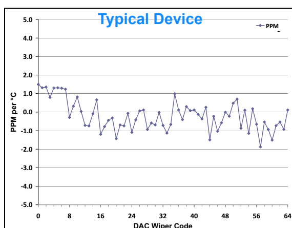
FIGURE 2-60: V_{OUT} Tempco vs. Code ( ((V_{OUT(+125C)} - V_{OUT(-40C)}) / V_{OUT(+25C, \text{Code}=FS)}) / 165) * 1,000,000 ), V_{DD} = 3.6\text{V} , V_{REF} = 1.65\text{V} .
