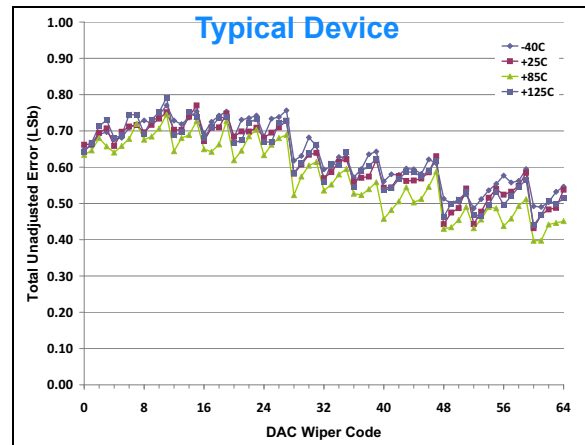
FIGURE 2-53: Total Unadjusted Error vs. Code and Temperature.
