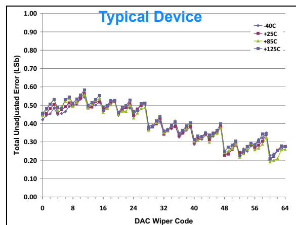
FIGURE 2-54: Total Unadjusted Error vs. Code and Temperature.
