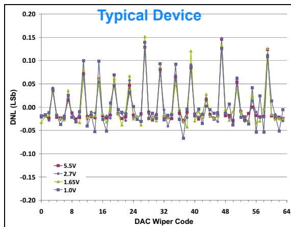
FIGURE 2-71: DNL vs. Code and V_{REF} V_{DD} = 5.5\text{V} , V_{REF} = 1\text{V} , 1.65V, 2.7V, and 5.5V, \text{Temp} = +25^\circ\text{C} .
