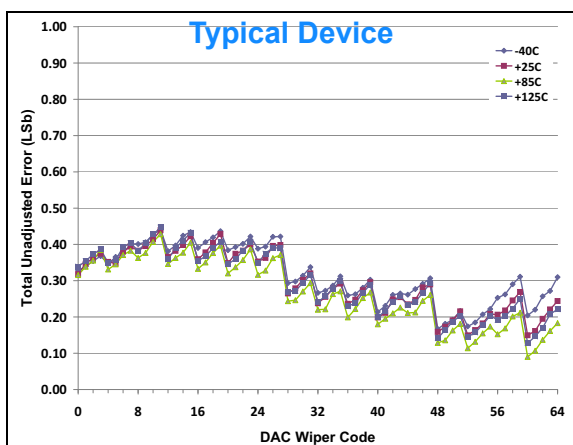
FIGURE 2-51: Total Unadjusted Error vs. Code and Temperature.
