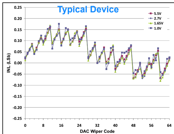
FIGURE 2-67: INL vs. Code and V_{REF} V_{DD} = 5.5\text{V} , V_{REF} = 1\text{V} , 1.65V, 2.7V, and 5.5V, \text{Temp} = +25^\circ\text{C} .
