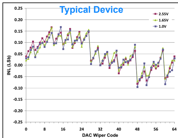
FIGURE 2-70: INL vs. Code and V_{REF} V_{DD} = 2.7\text{V} , V_{REF} = 1\text{V} , 1.65V, and 2.55V, \text{Temp} = +25^\circ\text{C} .
