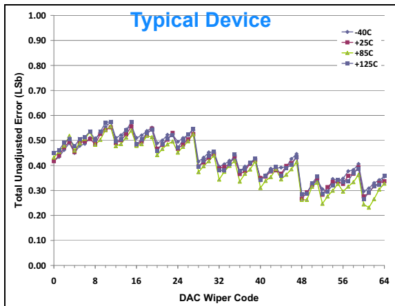
FIGURE 2-49: Total Unadjusted Error vs. Code and Temperature.
