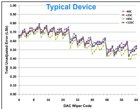
FIGURE 2-50: Total Unadjusted Error vs. Code and Temperature.
