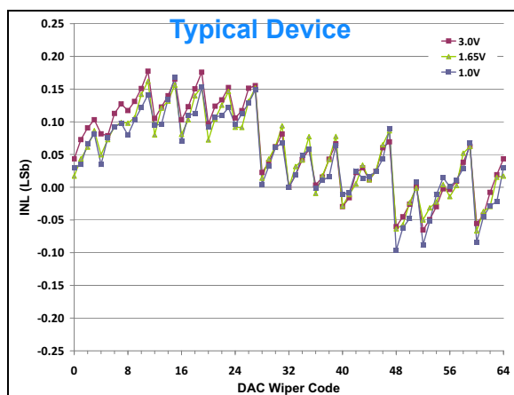
FIGURE 2-69: INL vs. Code and V_{REF} V_{DD} = 3.0\text{V} , V_{REF} = 1\text{V} , 1.65V, and 5.5V, \text{Temp} = +25^\circ\text{C} .
