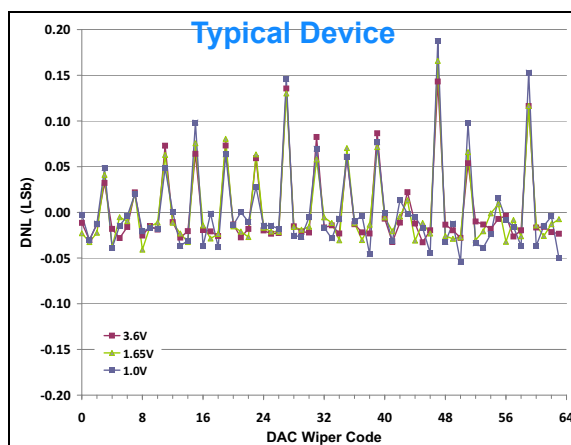
FIGURE 2-72: DNL vs. Code and V_{REF} V_{DD} = 3.6\text{V} , V_{REF} = 1\text{V} , 1.65V, and 3.6V, \text{Temp} = +25^\circ\text{C} .
