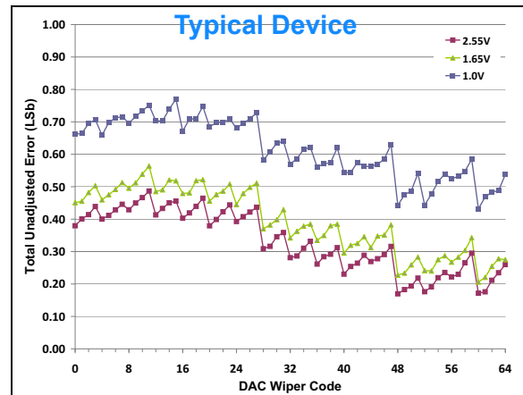
FIGURE 2-78: Total Unadjusted Error vs. Code and V_{REF} V_{DD} = 2.7\text{V} , V_{REF} = 1\text{V} , 1.65\text{V} , and 2.55\text{V} , \text{Temp} = +25^\circ\text{C} .
