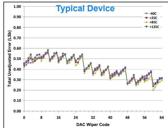
FIGURE 2-52: Total Unadjusted Error vs. Code and Temperature.
