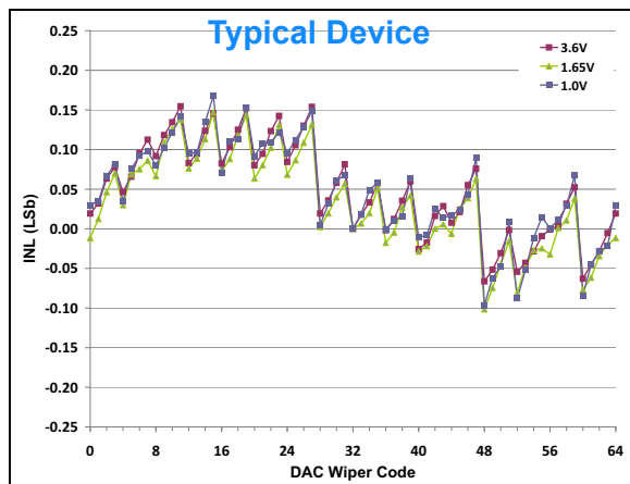
FIGURE 2-68: INL vs. Code and V_{REF} V_{DD} = 3.6\text{V} , V_{REF} = 1\text{V} , 1.65V, and 3.6V, \text{Temp} = +25^\circ\text{C} .
