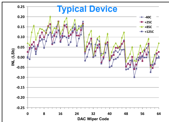
FIGURE 2-3: INL vs. Code and Temperature. V_{DD} = 5.5\text{V} , V_{REF} = 1.0\text{V} .
