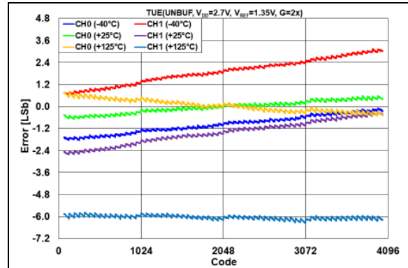
FIGURE 2-24: TUE ( V_{OUT} ) vs. DAC Code and Temperature, V_{DD} = 2.7\text{V} , V_{REF} = 1.35\text{V} , G = 2x .
