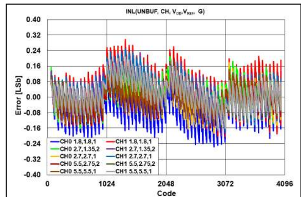
FIGURE 2-47: INL Error vs. DAC Code, Temperature = +25^\circ\text{C} .
