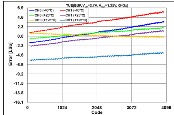
FIGURE 2-30: TUE(V_{OUT}) vs. DAC Code and Temperature, V_{REF} = 1.35\text{V} , V_{DD} = 2.7\text{V} , G = 2\text{x} .
