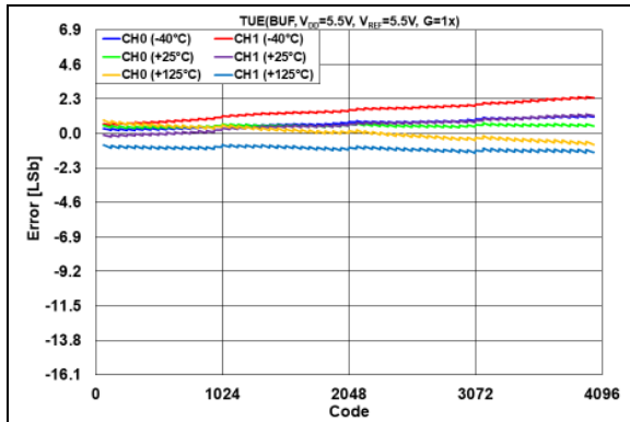
FIGURE 2-26: TUE(V_{OUT}) vs. DAC Code and Temperature, V_{REF} = V_{DD} = 5.5\text{V} , G = 1\text{x} .
