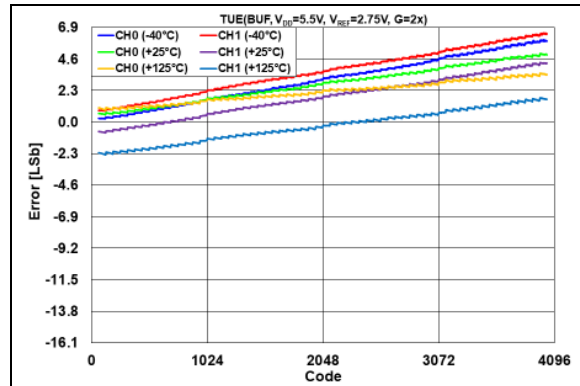
FIGURE 2-29: TUE(V_{OUT}) vs. DAC Code and Temperature, V_{REF} = 2.75\text{V} , V_{DD} = 5.5\text{V} , G = 2\text{x} .
