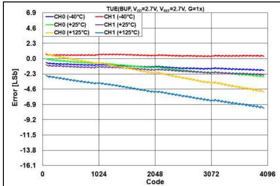
FIGURE 2-27: TUE(V_{OUT}) vs. DAC Code and Temperature, V_{REF} = V_{DD} = 2.7\text{V} , G = 1\text{x} .
