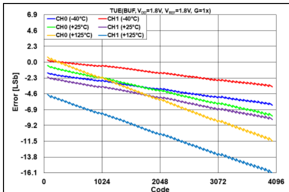
FIGURE 2-28: TUE(V_{OUT}) vs. DAC Code and Temperature, V_{REF} = V_{DD} = 2.7\text{V} , G = 1\text{x} .
