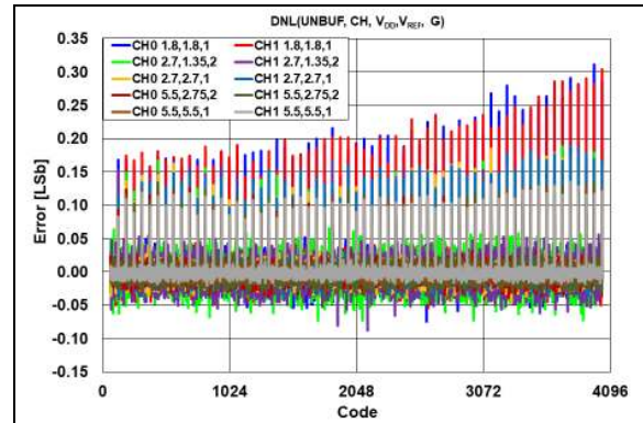
FIGURE 2-69: DNL Error vs. DAC Code, Temperature = +25^\circ\text{C} .
