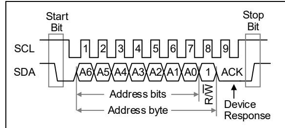
FIGURE 5-1: I 2 C Bus Connection Test.
