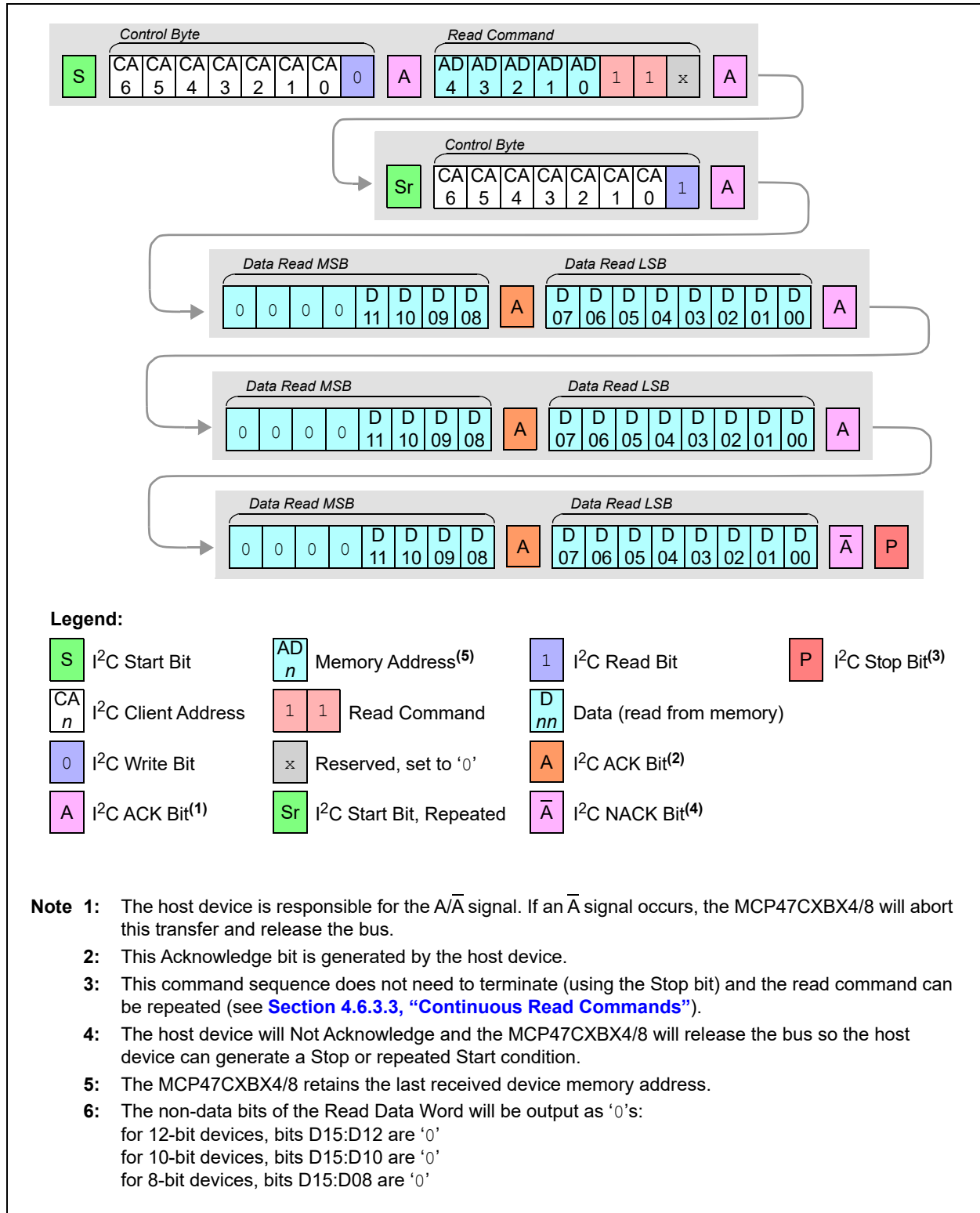
FIGURE 4-19: Continuous Read of Specified Address Command Format.
