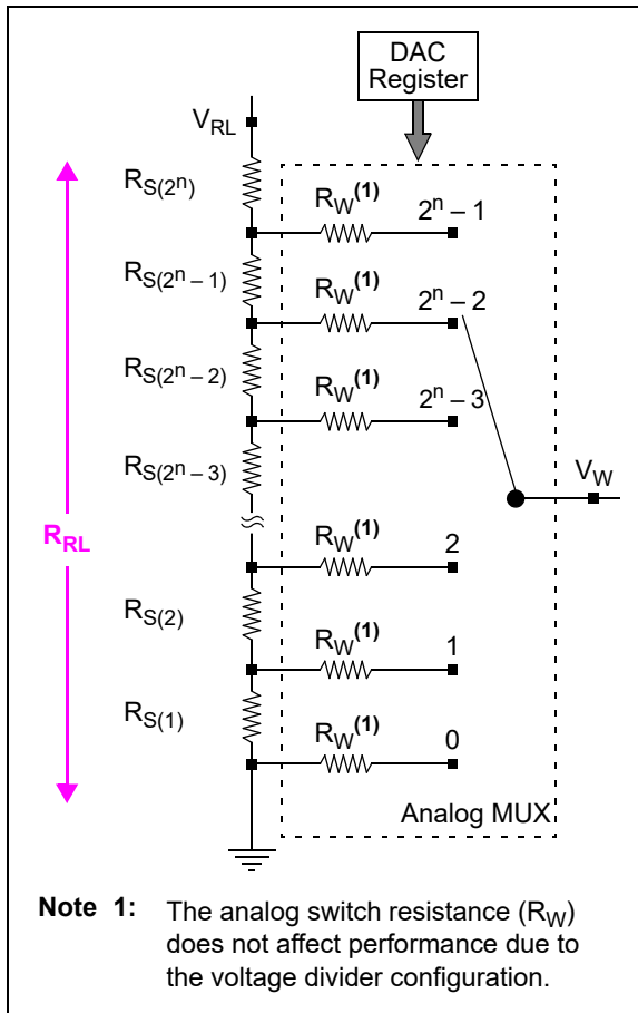
FIGURE 4-3: Resistor Ladder Model Block Diagram.
