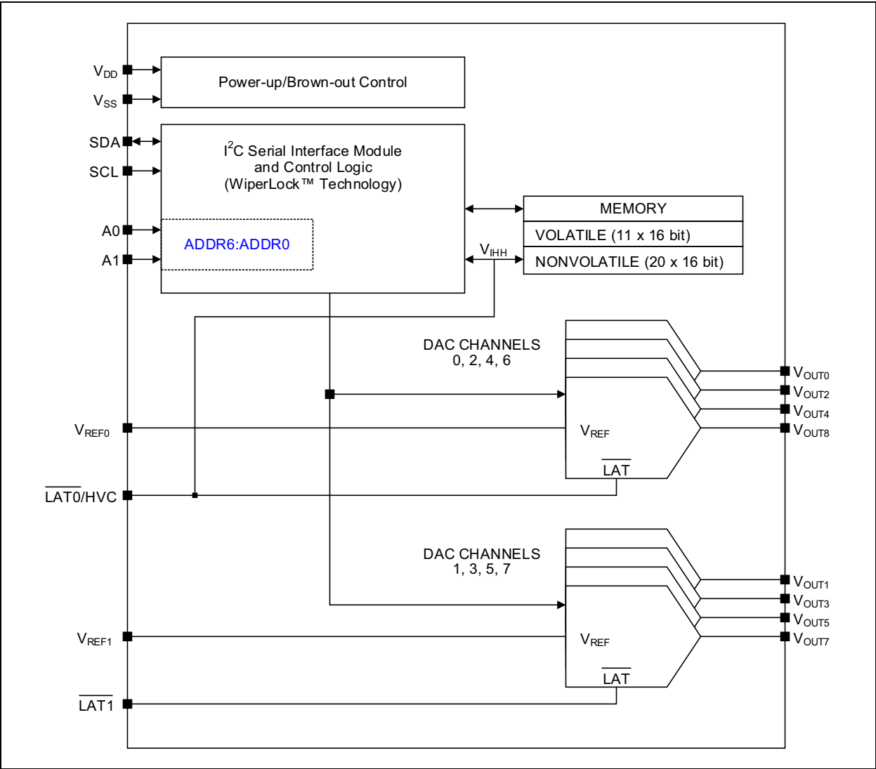
MCP47CXBX8 Block Diagram (Octal-Channel Output)
