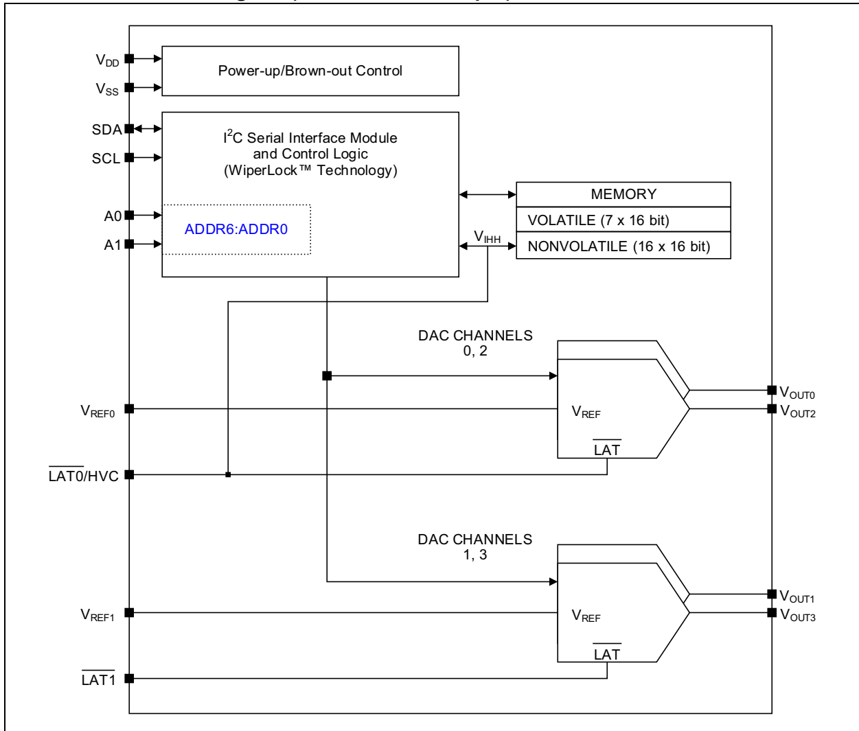
MCP47CXBX4 Block Diagram (Quad-Channel Output)
