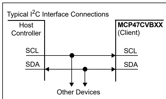
FIGURE 4-10: Typical I 2 C Interface.
