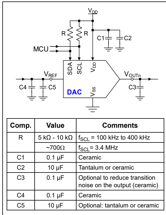
FIGURE 5-3: Example Circuit.
