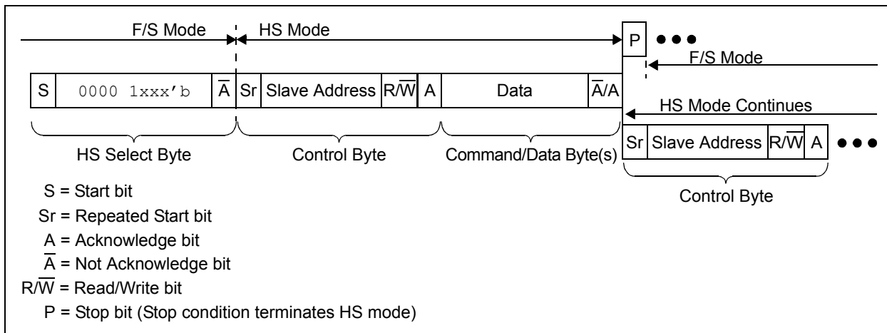
FIGURE B-10: HS Mode Sequence.
