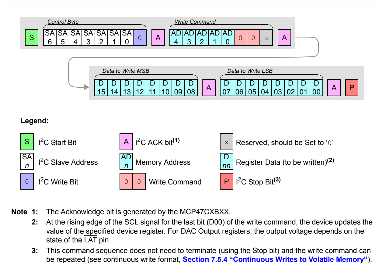
FIGURE 7-1: Write Random Address Command.
