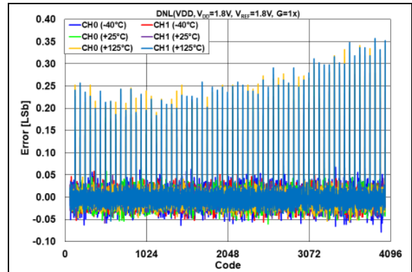
FIGURE 2-56: DNL Error vs. DAC Code and Temperature, V_{\text{REF}} = V_{DD} = 1.8\text{V} , G = 1\text{x} .
