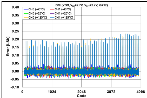
FIGURE 2-55: DNL Error vs. DAC Code and Temperature, V_{\text{REF}} = V_{DD} = 2.7\text{V} , G = 1\text{x} .
