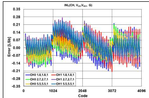
FIGURE 2-35: INL Error vs. DAC Code, Temperature = +25°C.
