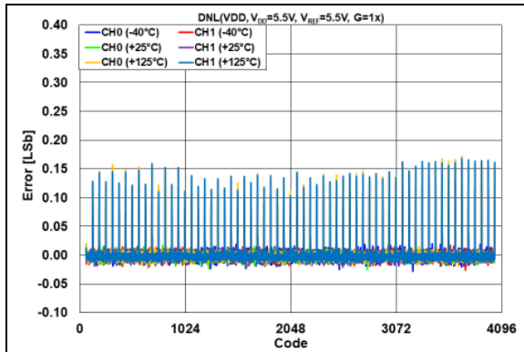
FIGURE 2-54: DNL Error vs. DAC Code and Temperature, V_{\text{REF}} = V_{DD} = 5.5\text{V} , G = 1\text{x} .
