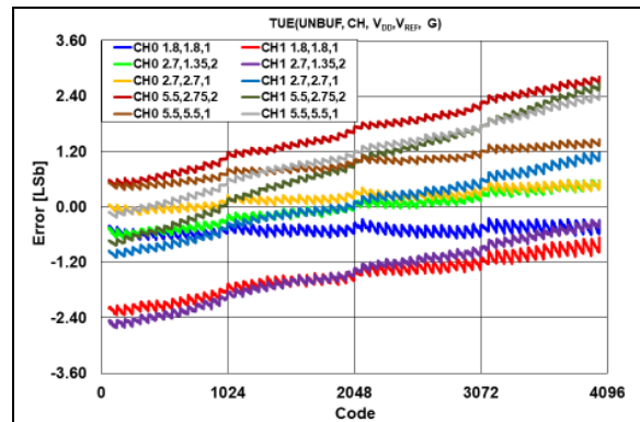
FIGURE 2-25: TUE ( V_{OUT} ) vs. DAC Code, Temperature = +25^\circ\text{C} .
