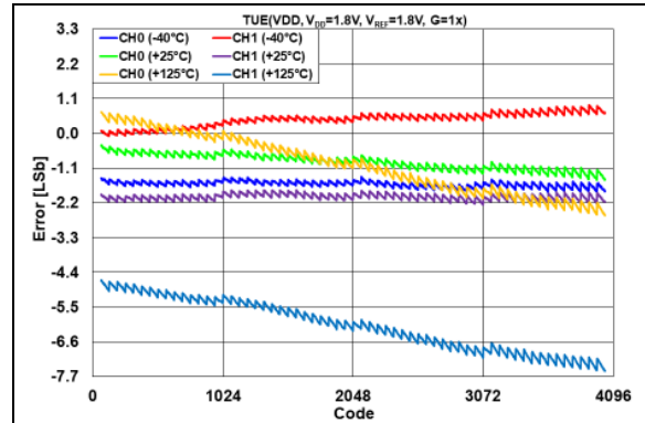
FIGURE 2-12: TUE ( V_{OUT} ) vs. DAC Code and Temperature, V_{REF} = V_{DD} = 1.8\text{V} , G = 1\text{x} .
