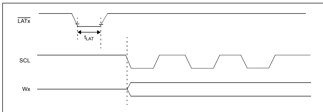
FIGURE 1-2: \overline{\text{LAT}} Pin Waveforms.
