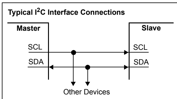
FIGURE B-1: Typical I 2 C Interface.
