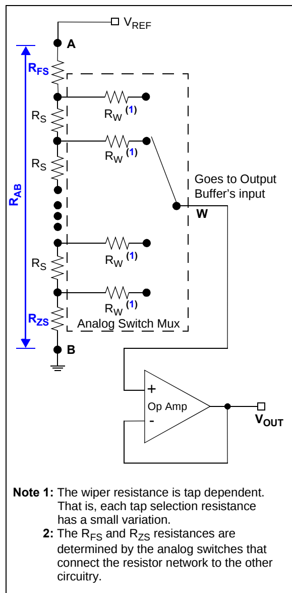
FIGURE 4-1: Resistor Network and Output Buffer Block Diagram.
