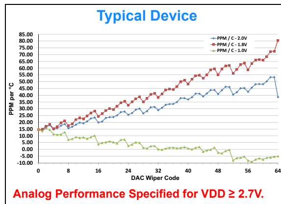
FIGURE 2-23: V_{OUT} Tempco vs. Code ( ((V_{OUT}(+125^\circ\text{C}) - V_{OUT}(-40^\circ\text{C})) / V_{OUT}(+25^\circ\text{C}, \text{Code=FS})) / 165) * 1,000,000 ), V_{DD} = 2.0\text{V} , V_{REF} = 2.0\text{V} , 1.8\text{V} , and 1.0\text{V} .
