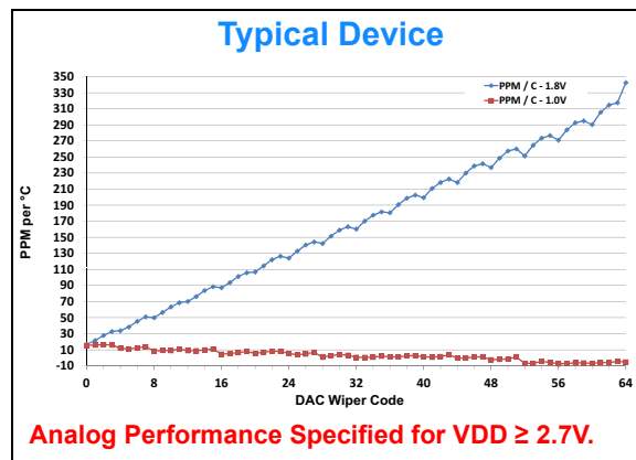
FIGURE 2-24: V_{OUT} Tempco vs. Code ( ((V_{OUT}(+125^\circ\text{C}) - V_{OUT}(-40^\circ\text{C})) / V_{OUT}(+25^\circ\text{C}, \text{Code=FS})) / 165) * 1,000,000 ), V_{DD} = 1.8\text{V} , V_{REF} = 1.6\text{V} , and 1.0\text{V} .
