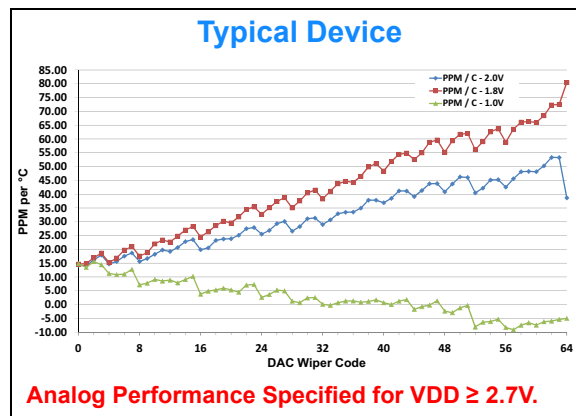
FIGURE 2-23: V_{OUT} Tempco vs. Code ( ((V_{OUT}(+125^\circ\text{C}) - V_{OUT}(-40^\circ\text{C})) / V_{OUT}(+25^\circ\text{C}, \text{Code=FS})) / 165) * 1,000,000 ), V_{DD} = 2.0\text{V} , V_{REF} = 2.0\text{V} , 1.8\text{V} , and 1.0\text{V} .
