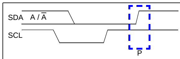
FIGURE 5-6: Stop Condition Receive or Transmit Mode.
