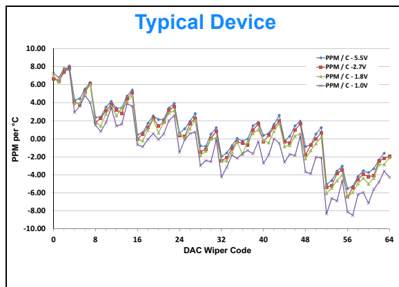
FIGURE 2-21: V_{OUT} Tempco vs. Code ( ((V_{OUT}(+125^\circ\text{C}) - V_{OUT}(-40^\circ\text{C})) / V_{OUT}(+25^\circ\text{C}, \text{Code=FS})) / 165) * 1,000,000 ), V_{DD} = 5.5\text{V} , V_{REF} = 5.5\text{V} , 2.7\text{V} , 1.8\text{V} , and 1.0\text{V} .
