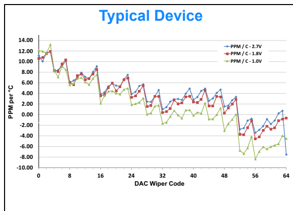
FIGURE 2-22: V_{OUT} Tempco vs. Code ( ((V_{OUT}(+125^\circ\text{C}) - V_{OUT}(-40^\circ\text{C})) / V_{OUT}(+25^\circ\text{C}, \text{Code=FS})) / 165) * 1,000,000 ), V_{DD} = 2.7\text{V} , V_{REF} = 2.7\text{V} , 1.8\text{V} , and 1.0\text{V} .
