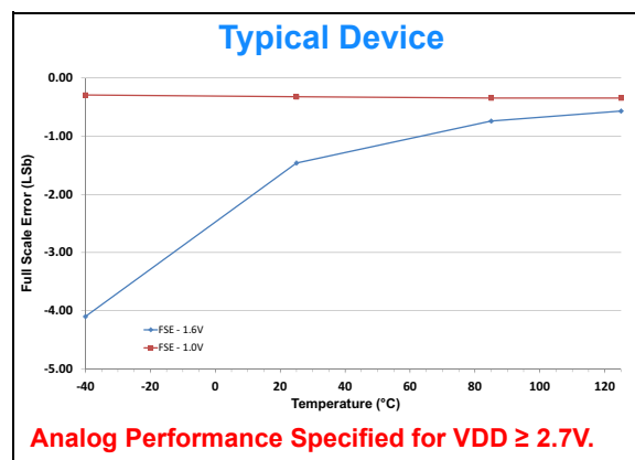
FIGURE 2-12: Full Scale Error (FSE) vs. Temperature. V_{DD} = 1.8\text{V} , V_{REF} = 1.6\text{V} , and 1.0\text{V} .
