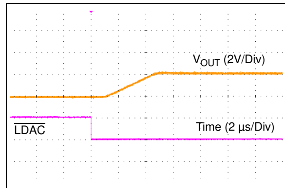
FIGURE 2-28: Full Scale Settling Time ( V_{REF} = \text{Internal} , V_{DD} = 5\text{V} , \overline{\text{LDAC}} = 1 , Gain = \times 1 , Code Change: 000\text{h} to \text{FFFh} ).
