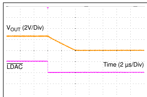
FIGURE 2-30: Half Scale Settling Time ( V_{REF} = V_{DD} , V_{DD} = 5\text{V} , \overline{\text{LDAC}} = 1 , Code Change: 7\text{FFh} to 000\text{h} ).
