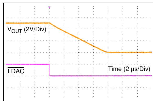
FIGURE 2-29: Full Scale Settling Time ( V_{REF} = V_{DD} , V_{DD} = 5\text{V} , \overline{\text{LDAC}} = 1 , Code Change: \text{FFFh} to 000\text{h} ).
