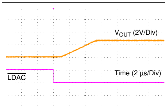
FIGURE 2-27: Half Scale Settling Time ( V_{REF} = V_{DD} , V_{DD} = 5\text{V} , \overline{\text{LDAC}} = 1 , Code Change: 000\text{h} to 7\text{FFh} ).
