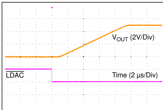
FIGURE 2-26: Full Scale Settling Time ( V_{REF} = V_{DD} , V_{DD} = 5\text{V} , \overline{\text{LDAC}} = 1 , Code Change: 000\text{h} to \text{FFFh} ).
