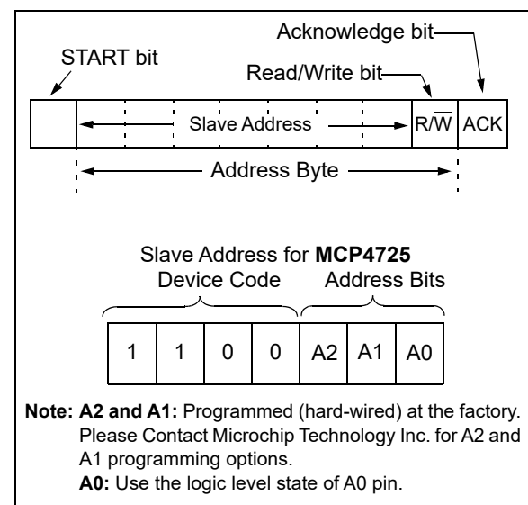
FIGURE 7-1: Device Addressing.
