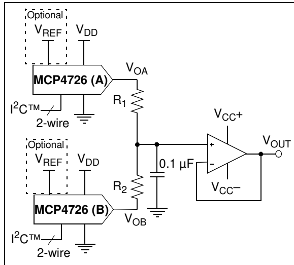
FIGURE 8-7: Simple Double Precision DAC using MCP4726.
