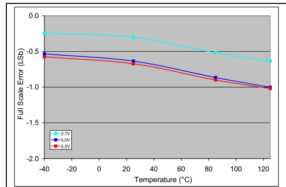
FIGURE 2-54: Full-Scale Error (FSE) vs. Temperature (MCP4706).
