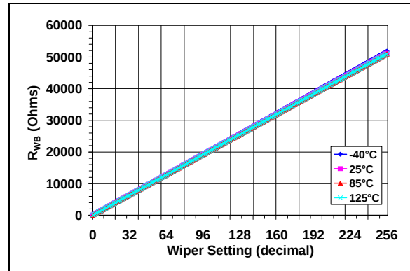
FIGURE 2-33: 50 k \Omega – R_{WB} ( \Omega ) vs. Wiper Setting and Ambient Temperature.
