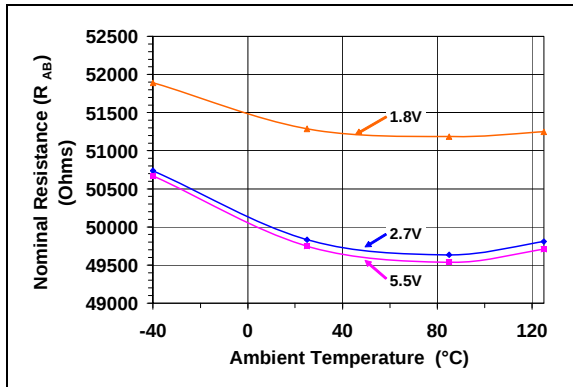
FIGURE 2-32: 50 k \Omega – Nominal Resistance ( \Omega ) vs. Ambient Temperature and V_{DD} .
