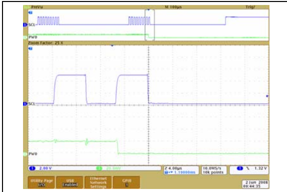
FIGURE 2-45: 100 kΩ – Low-Voltage Decrement Wiper Settling Time ( V_{DD} = 5.5\text{V} ) ( 1\text{ }\mu\text{s/Div} ).
