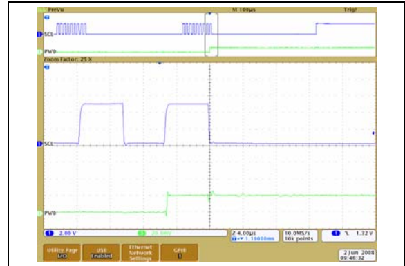
FIGURE 2-47: 100 kΩ – Low-Voltage Increment Wiper Settling Time ( V_{DD} = 5.5\text{V} ) ( 1\text{ }\mu\text{s/Div} ).
