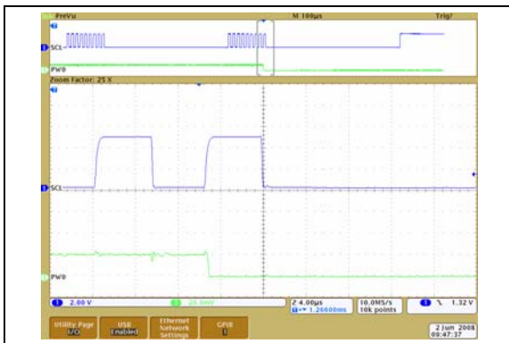
FIGURE 2-46: 100 kΩ – Low-Voltage Decrement Wiper Settling Time ( V_{DD} = 2.7\text{V} ) ( 1\text{ }\mu\text{s/Div} ).
