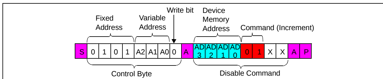
FIGURE 7-9: I 2 C Disable Command Sequence.
