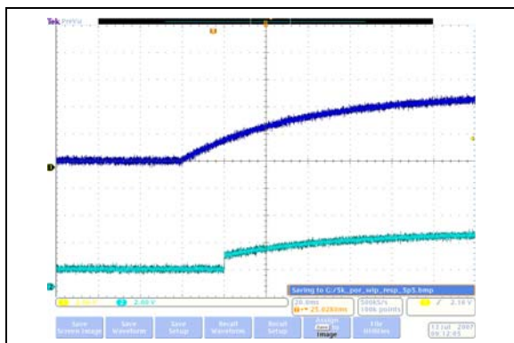
FIGURE 2-14: 5\text{ k}\Omega – Power-Up Wiper Response Time ( 20\text{ ms/Div} ).
