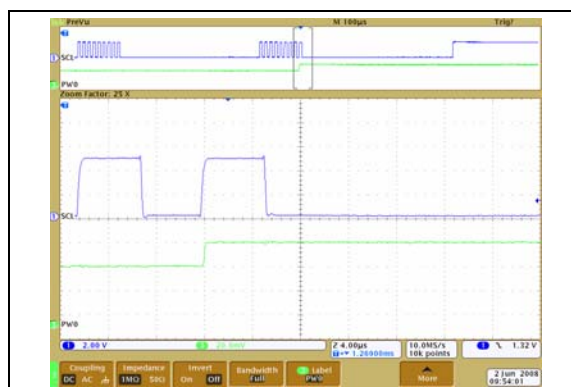
FIGURE 2-16: 5\text{ k}\Omega – Low-Voltage Increment Wiper Settling Time ( V_{DD} = 2.7\text{V} ) ( 1\text{ }\mu\text{s/Div} ).
