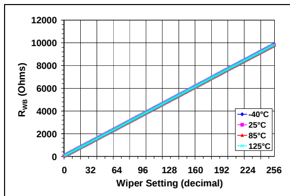
FIGURE 2-26: 10 kΩ – R_{WB} (Ω) vs. Wiper Setting and Ambient Temperature.
