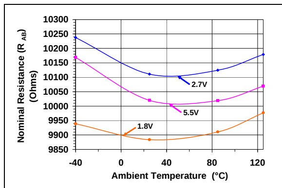
FIGURE 2-25: 10 kΩ – Nominal Resistance (Ω) vs. Ambient Temperature and V_{DD} .
