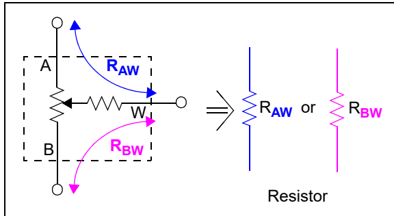
FIGURE 5-8: Rheostat Configuration.
