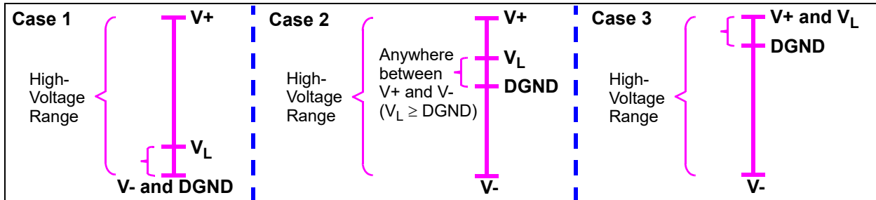
FIGURE 4-2: Voltage Ranges.
