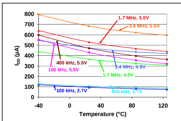
FIGURE 2-1: Device Current ( I_{DD} ) vs. f^2\text{C} Frequency ( f_{\text{SCL}} ) and Ambient Temperature ( V_{DD} = 2.7\text{V} and 5.5\text{V} ).
