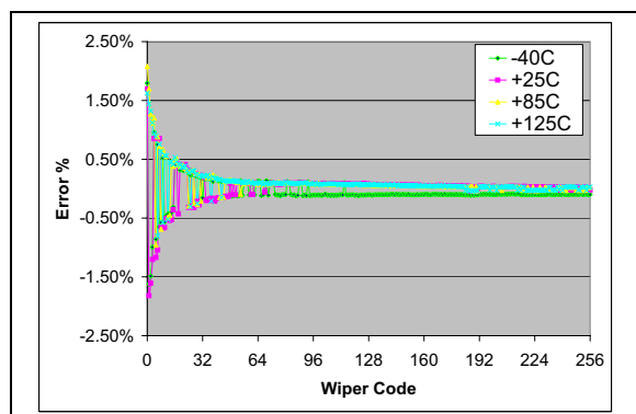
FIGURE 2-13: 5 kΩ – Worst Case R_{BW} from Average R_{BW} ( R_{BW0} - R_{BW3} ) Error (%) vs. Wiper Setting and Temperature ( V_{DD} = 5.5\text{V} , I_W = 190\text{ }\mu\text{A} ).
