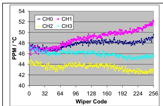
FIGURE 2-15: 5 kΩ – R_{WB} PPM/ ^\circ\text{C} vs. Wiper Setting. ( R_{BW(\text{code}=n, 125^\circ\text{C})} - R_{BW(\text{code}=n, -40^\circ\text{C})} / R_{BW(\text{code}=256, 25^\circ\text{C})} / 165^\circ\text{C} * 1,000,000 ) ( V_{DD} = 5.5\text{V} , I_W = 190\text{ }\mu\text{A} ).
