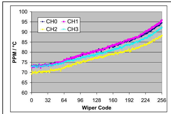
FIGURE 2-16: 5 kΩ – R_{WB} PPM/ ^\circ\text{C} vs. Wiper Setting. ( R_{BW(\text{code}=n, 125^\circ\text{C})} - R_{BW(\text{code}=n, -40^\circ\text{C})} / R_{BW(\text{code}=256, 25^\circ\text{C})} / 165^\circ\text{C} * 1,000,000 ) ( V_{DD} = 3.0\text{V} , I_W = 190\text{ }\mu\text{A} ).
