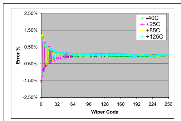
FIGURE 2-14: 5 kΩ – Worst Case R_{BW} from Average R_{BW} ( R_{BW0} - R_{BW3} ) Error (%) vs. Wiper Setting and Temperature ( V_{DD} = 3.0\text{V} , I_W = 190\text{ }\mu\text{A} ).
