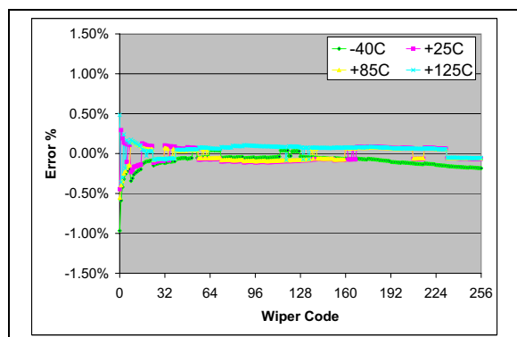
FIGURE 2-29: 10 k \Omega – Worst Case R_{BW} from Average R_{BW} ( R_{BW0} - R_{BW3} ) Error (%) vs. Wiper Setting and Temperature ( V_{DD} = 5.5\text{V} , I_W = 150\text{ }\mu\text{A} ).
