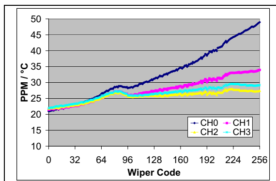
FIGURE 2-31: 10 k \Omega – R_{WB} PPM/ ^\circ\text{C} vs. Wiper Setting. ( R_{BW(\text{code}=n, 125^\circ\text{C})} - R_{BW(\text{code}=n, -40^\circ\text{C})} / R_{BW(\text{code}=256, 25^\circ\text{C})} / 165^\circ\text{C} * 1,000,000 ) ( V_{DD} = 5.5\text{V} , I_W = 150\text{ }\mu\text{A} ).
