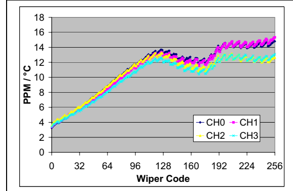
FIGURE 2-62: 100 k \Omega – R_{WB} PPM/ ^\circ\text{C} vs. Wiper Setting. ( R_{BW(\text{code}=n, 125^\circ\text{C})} - R_{BW(\text{code}=n, -40^\circ\text{C})} / R_{BW(\text{code}=256, 25^\circ\text{C})} / 165^\circ\text{C} * 1,000,000 ) ( V_{DD} = 3.0\text{V} , I_W = 24\text{ }\mu\text{A} ).
