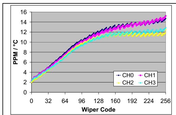
FIGURE 2-61: 100 k \Omega – R_{WB} PPM/ ^\circ\text{C} vs. Wiper Setting. ( R_{BW(\text{code}=n, 125^\circ\text{C})} - R_{BW(\text{code}=n, -40^\circ\text{C})} / R_{BW(\text{code}=256, 25^\circ\text{C})} / 165^\circ\text{C} * 1,000,000 ) ( V_{DD} = 5.5\text{V} , I_W = 45\text{ }\mu\text{A} ).
