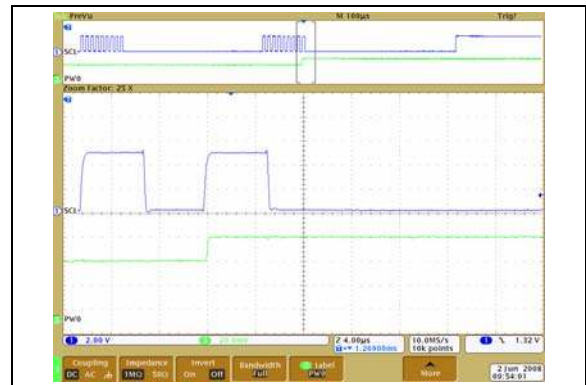
FIGURE 2-21: 5\text{ k}\Omega – Low-Voltage Increment Wiper Settling Time ( V_{DD} = 5.5\text{V} ) ( 1\text{ }\mu\text{s}/\text{Div} ).
