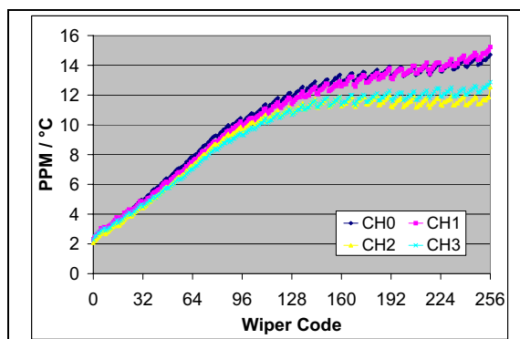
FIGURE 2-61: 100 k \Omega – R_{WB} PPM/ ^\circ\text{C} vs. Wiper Setting. ( R_{BW}(\text{code}=n, 125^\circ\text{C}) - R_{BW}(\text{code}=n, -40^\circ\text{C}) ) / R_{BW}(\text{code} = 256, 25^\circ\text{C}) / 165^\circ\text{C} * 1,000,000 ) ( V_{DD} = 5.5\text{V} , I_W = 45\text{ }\mu\text{A} ).
