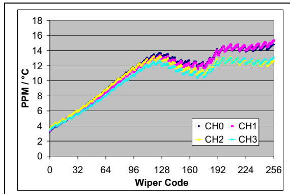
FIGURE 2-62: 100 k \Omega – R_{WB} PPM/ ^\circ\text{C} vs. Wiper Setting. ( R_{BW}(\text{code}=n, 125^\circ\text{C}) - R_{BW}(\text{code}=n, -40^\circ\text{C}) ) / R_{BW}(\text{code} = 256, 25^\circ\text{C}) / 165^\circ\text{C} * 1,000,000 ) ( V_{DD} = 3.0\text{V} , I_W = 24\text{ }\mu\text{A} ).
