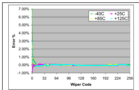
FIGURE 2-44: 50 k \Omega – Worst Case R_{BW} from Average R_{BW} ( R_{BW0} - R_{BW3} ) Error (%) vs. Wiper Setting and Temperature ( V_{DD} = 5.5\text{V} , I_W = 90\text{ }\mu\text{A} ).
