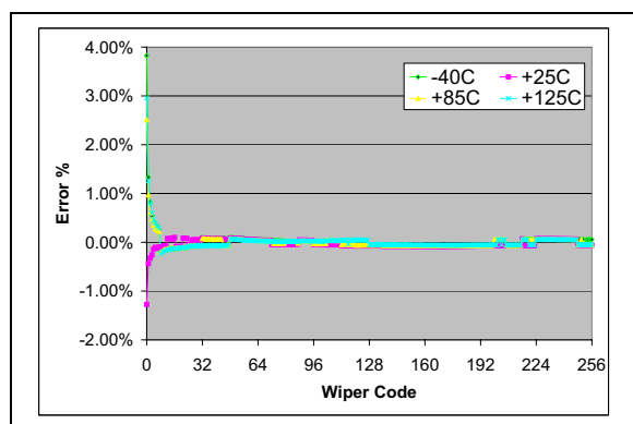
FIGURE 2-45: 50 k \Omega – Worst Case R_{BW} from Average R_{BW} ( R_{BW0} - R_{BW3} ) Error (%) vs. Wiper Setting and Temperature ( V_{DD} = 3.0\text{V} , I_W = 48\text{ }\mu\text{A} ).
