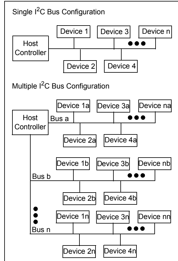
FIGURE 8-5: Typical Application I 2 C Bus Configurations.
