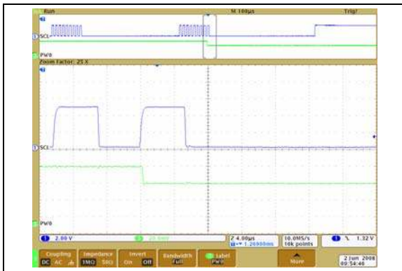
FIGURE 2-18: 5\text{ k}\Omega – Low-Voltage Decrement Wiper Settling Time ( V_{DD} = 5.5\text{V} ) ( 1\text{ }\mu\text{s}/\text{Div} ).
