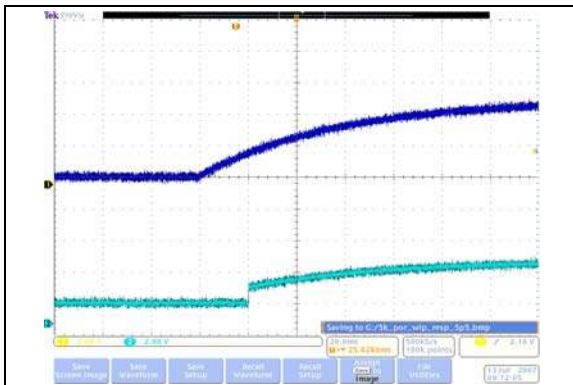
FIGURE 2-19: 5\text{ k}\Omega – Power-Up Wiper Response Time ( 20\text{ ms}/\text{Div} ).
