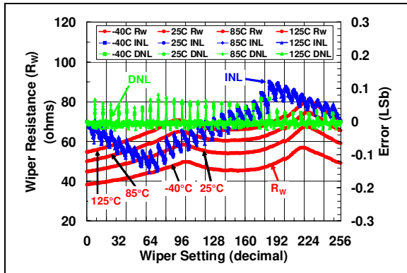
FIGURE 2-6: 5 kΩ Pot Mode – R_W (Ω), INL (LSb), DNL (LSb) vs. Wiper Setting and Ambient Temperature ( V_{DD} = 5.5\text{V} ).
