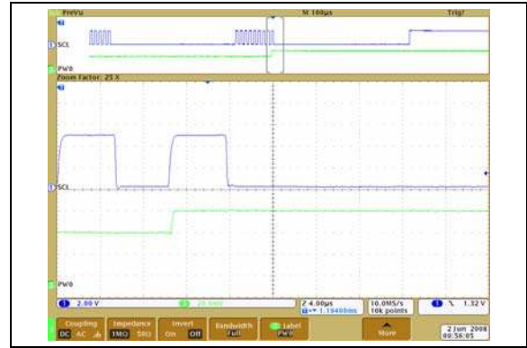
FIGURE 2-20: 5\text{ k}\Omega – Low-Voltage Increment Wiper Settling Time ( V_{DD} = 2.7\text{V} ) ( 1\text{ }\mu\text{s}/\text{Div} ).
