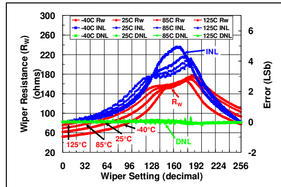
FIGURE 2-9: 5 kΩ Rheo Mode – R_W (Ω), INL (LSb), DNL (LSb) vs. Wiper Setting and Ambient Temperature ( V_{DD} = 3.0\text{V} ).
