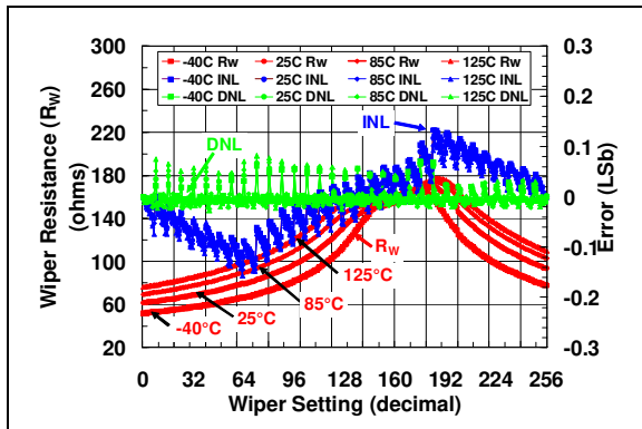
FIGURE 2-7: 5 kΩ Pot Mode – R_W (Ω), INL (LSb), DNL (LSb) vs. Wiper Setting and Ambient Temperature ( V_{DD} = 3.0\text{V} ).
