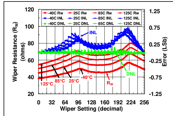
FIGURE 2-8: 5 kΩ Rheo Mode – R_W (Ω), INL (LSb), DNL (LSb) vs. Wiper Setting and Ambient Temperature ( V_{DD} = 5.5\text{V} ).
