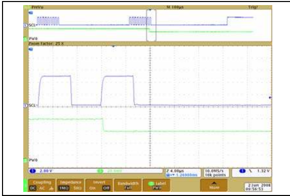
FIGURE 2-17: 5\text{ k}\Omega – Low-Voltage Decrement Wiper Settling Time ( V_{DD} = 2.7\text{V} ) ( 1\text{ }\mu\text{s}/\text{Div} ).
