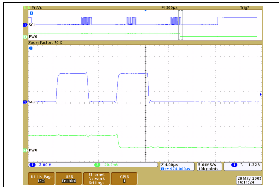
FIGURE 2-62: 50\text{ k}\Omega – Low-Voltage Decrement Wiper Settling Time ( V_{DD} = 2.7\text{V} ) ( 1\text{ }\mu\text{s}/\text{Div} ).
