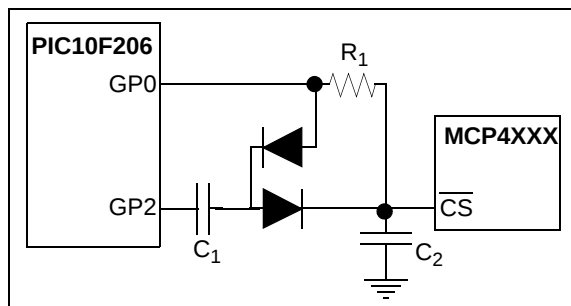
FIGURE 8-4: MCP4XXX Non-volatile Digital Potentiometer Evaluation Board (MCP402XEV) implementation to generate the V_{IH} voltage.
