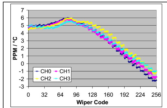
FIGURE 2-59: 50 kΩ – R_{WB} PPM/°C vs. Wiper Setting. ( R_{BW(\text{code}=n, 125^\circ\text{C})} - R_{BW(\text{code}=n, -40^\circ\text{C})} / R_{BW(\text{code} = 256, 25^\circ\text{C}) / 165^\circ\text{C} * 1,000,000 ) ( V_{DD} = 5.5\text{V} , I_W = 90\text{ }\mu\text{A} ).
