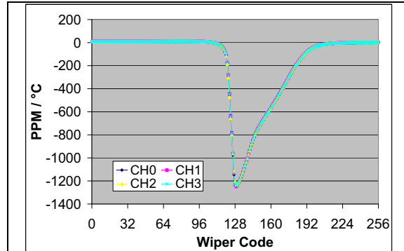
FIGURE 2-60: 50 kΩ – R_{WB} PPM/°C vs. Wiper Setting. ( R_{BW(\text{code}=n, 125^\circ\text{C})} - R_{BW(\text{code}=n, -40^\circ\text{C})} / R_{BW(\text{code} = 256, 25^\circ\text{C}) / 165^\circ\text{C} * 1,000,000 ) ( V_{DD} = 3.0\text{V} , I_W = 48\text{ }\mu\text{A} ).
