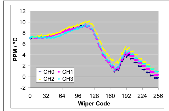
FIGURE 2-60: 50 kΩ – R_{WB} PPM/°C vs. Wiper Setting. ( R_{BW(\text{code}=n, 125^\circ\text{C})} - R_{BW(\text{code}=n, -40^\circ\text{C})} / R_{BW(\text{code} = 256, 25^\circ\text{C}) / 165^\circ\text{C} * 1,000,000 ) ( V_{DD} = 3.0\text{V} , I_W = 48\text{ }\mu\text{A} ).
