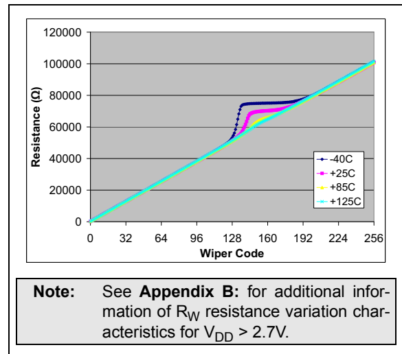
FIGURE 2-75: 100\text{ k}\Omega – R_{WB} ( \Omega ) vs. Wiper Setting and Ambient Temperature ( V_{DD} = 1.8\text{V} , I_W = 15\text{ }\mu\text{A} ).
