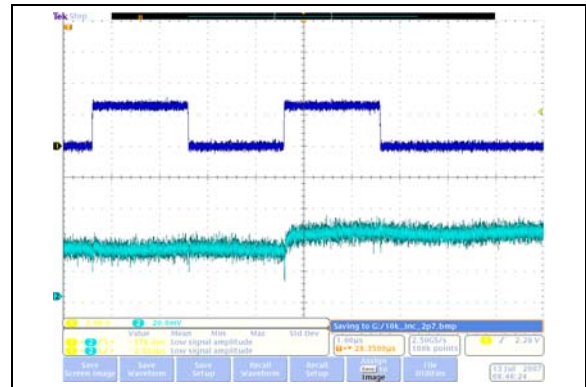
FIGURE 2-25: 10 k \Omega – Low-Voltage Increment Wiper Settling Time ( V_{DD} = 2.7\text{V} ) ( 1\text{ }\mu\text{s}/\text{Div} ).
