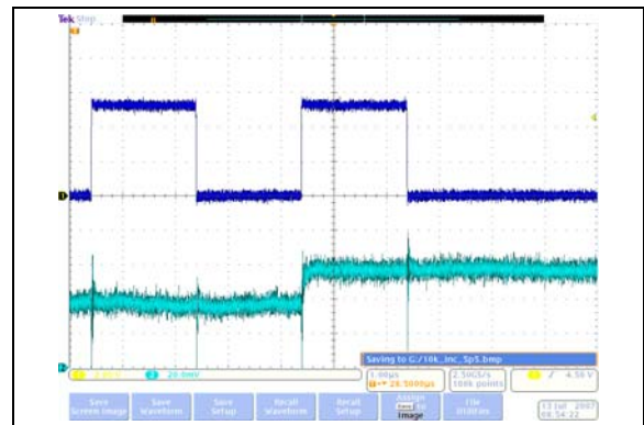
FIGURE 2-26: 10 k \Omega – Low-Voltage Increment Wiper Settling Time ( V_{DD} = 5.5\text{V} ) ( 1\text{ }\mu\text{s}/\text{Div} ).
