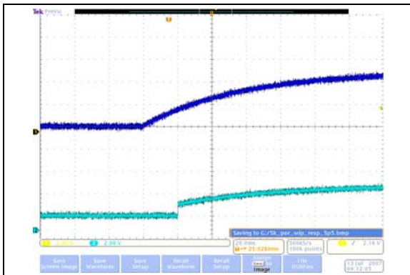
FIGURE 2-15: 5 kΩ – Power-Up Wiper Response Time ( 20\text{ ms/Div} ).
