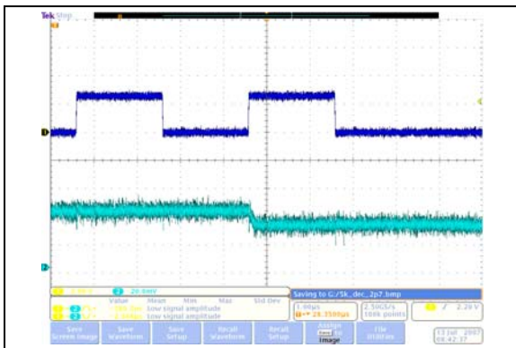
FIGURE 2-14: 5 kΩ – Low-Voltage Decrement Wiper Settling Time ( V_{DD} = 2.7\text{V} ) ( 1\text{ }\mu\text{s/Div} ).
