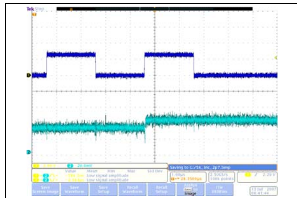
FIGURE 2-17: 5 kΩ – Low-Voltage Increment Wiper Settling Time ( V_{DD} = 2.7\text{V} ) ( 1\text{ }\mu\text{s/Div} ).
