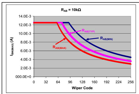
FIGURE 5-4: Maximum I_{BW} Vs. Wiper Code – 10 k \Omega .
