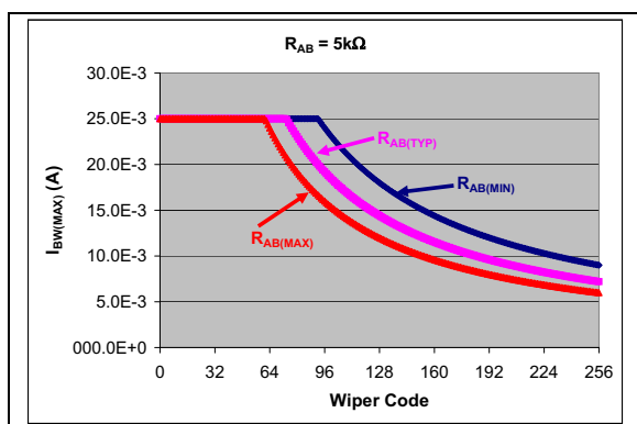
FIGURE 5-3: Maximum I_{BW} Vs. Wiper Code – 5 k \Omega .
