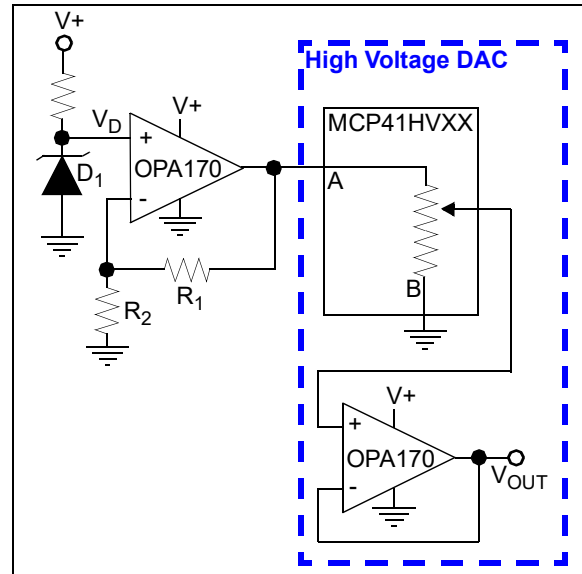
FIGURE 8-4: High-Voltage DAC.
