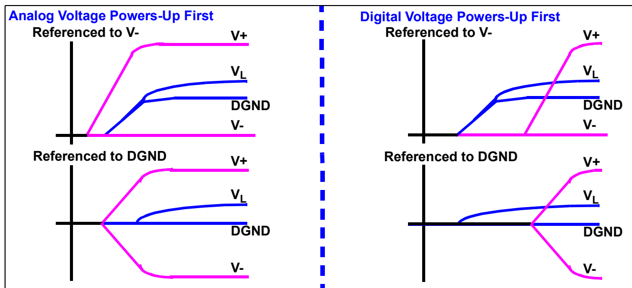
FIGURE 4-1: Power-On Sequences.
