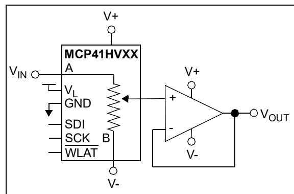
FIGURE 8-6: Audio Volume Control.
