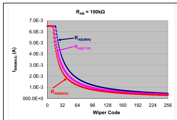
FIGURE 5-6: Maximum I_{BW} Vs. Wiper Code – 100 k \Omega .
