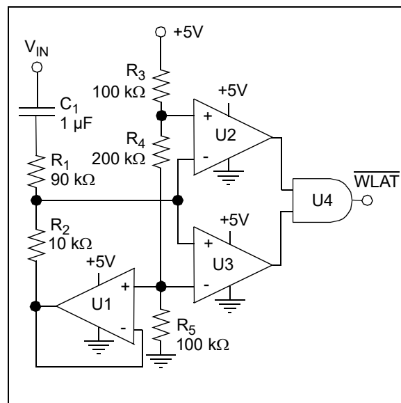
FIGURE 8-7: Referenced Voltage Crossing Detect.
