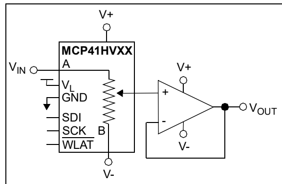
FIGURE 8-6: Audio Volume Control.
