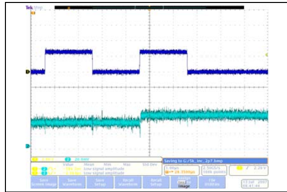
FIGURE 2-17: 5 kΩ – Low-Voltage Increment Wiper Settling Time ( V_{DD} = 2.7\text{V} ) (1 μs/Div).
