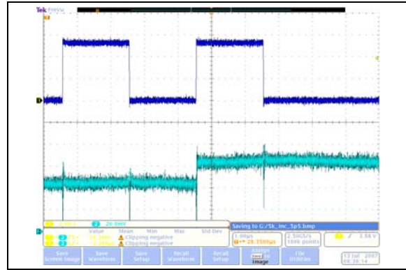
FIGURE 2-16: 5 kΩ – Low-Voltage Increment Wiper Settling Time ( V_{DD} = 5.5\text{V} ) (1 μs/Div).
