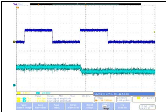
FIGURE 2-14: 5 kΩ – Low-Voltage Decrement Wiper Settling Time ( V_{DD} = 2.7\text{V} ) (1 μs/Div).
