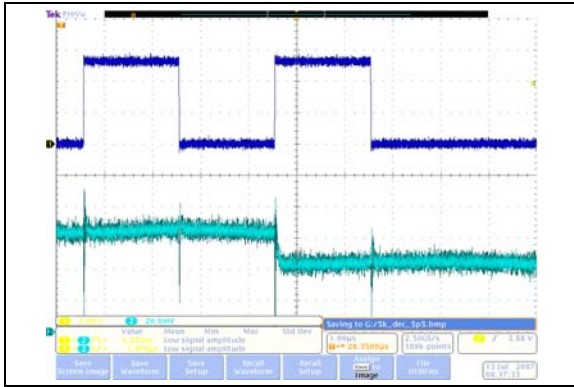
FIGURE 2-13: 5 kΩ – Low-Voltage Decrement Wiper Settling Time ( V_{DD} = 5.5\text{V} ) (1 μs/Div).
