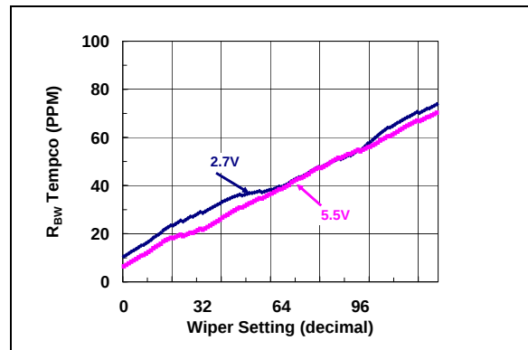
FIGURE 2-48: 50 kΩ : R_{BW} Tempco \Delta R_{BW} / \Delta T vs. Code.
